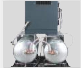
· KK variant with automatic condensate drain as a factory standard · for reliable and economic condensate draining without unnecessary compressed air loss
