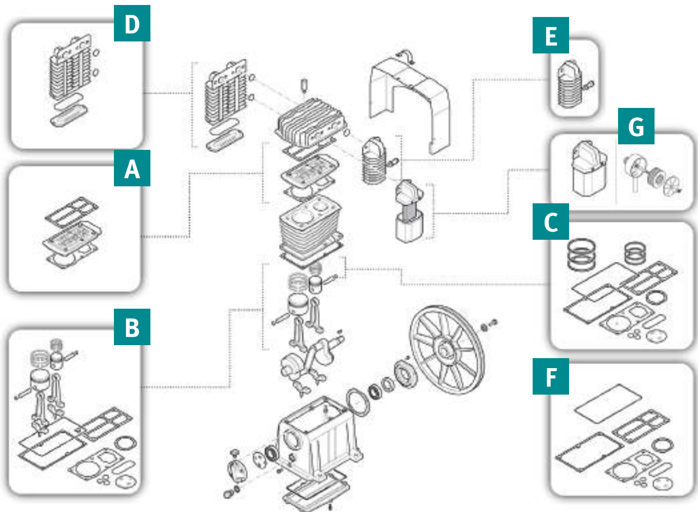
Two-stage unit
